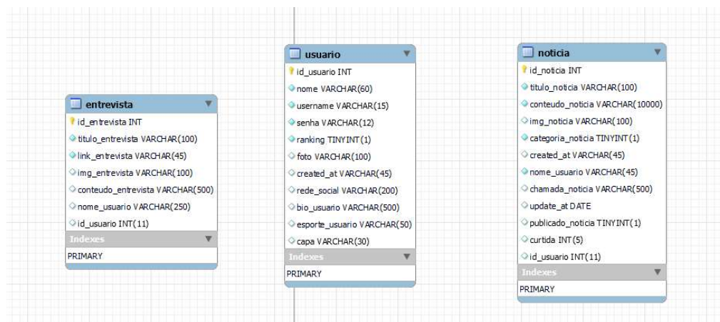
Figure 13: DER
