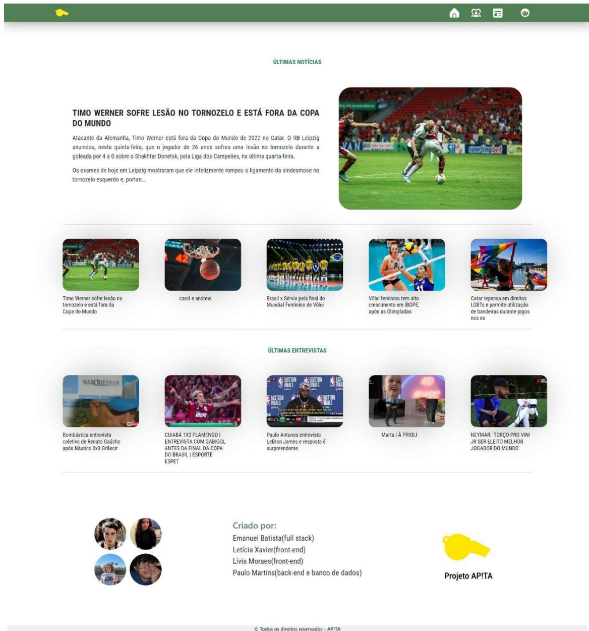
Figure 1: Tela inicial
