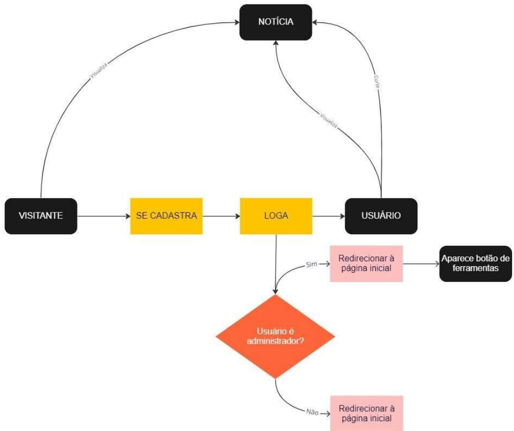
Figure 14: Fluxograma
