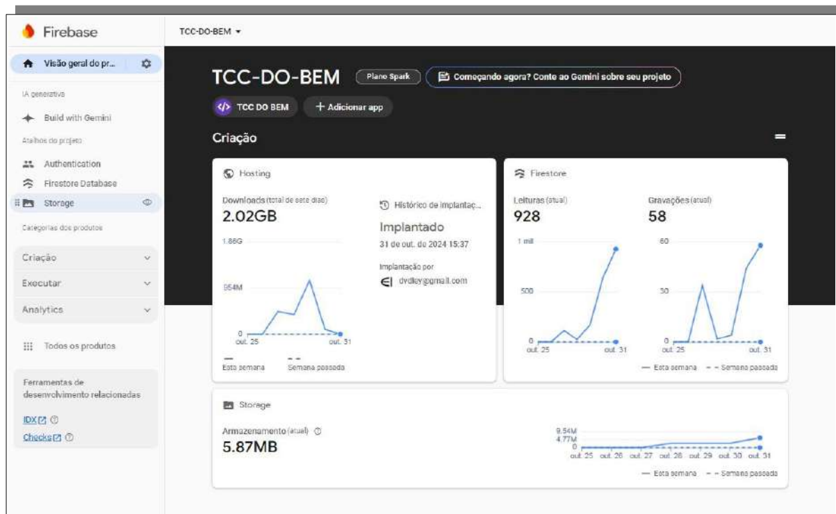
Figura 17 – Firebase
