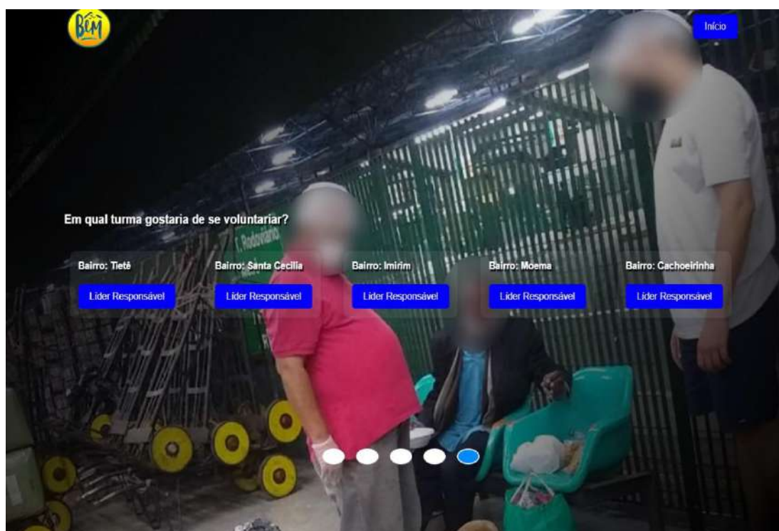
Figura 10 – Home Page
